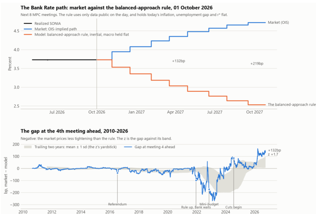
Figure 3. GBP: the market path against the balanced-approach rule, and the gap at the fourth meeting ahead.
